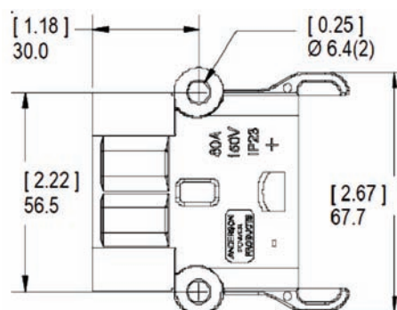
MALE
