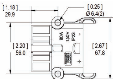
FEMALE
