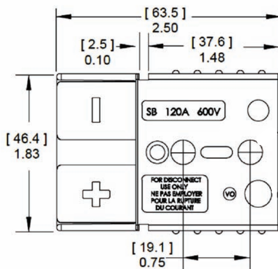
SB120
